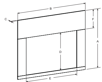
SH1BL Universal Shroud (for insert installations only, drawing not to scale)
